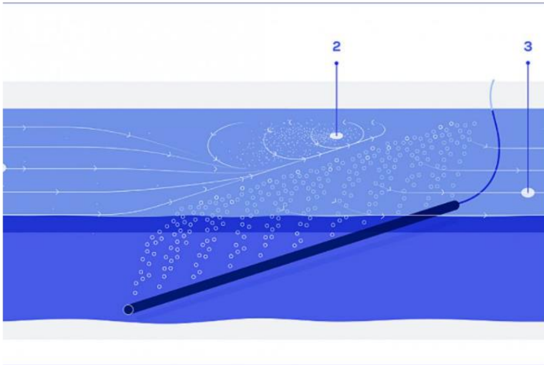
Figure 3. Schematic diagram of creating an aeration screen
